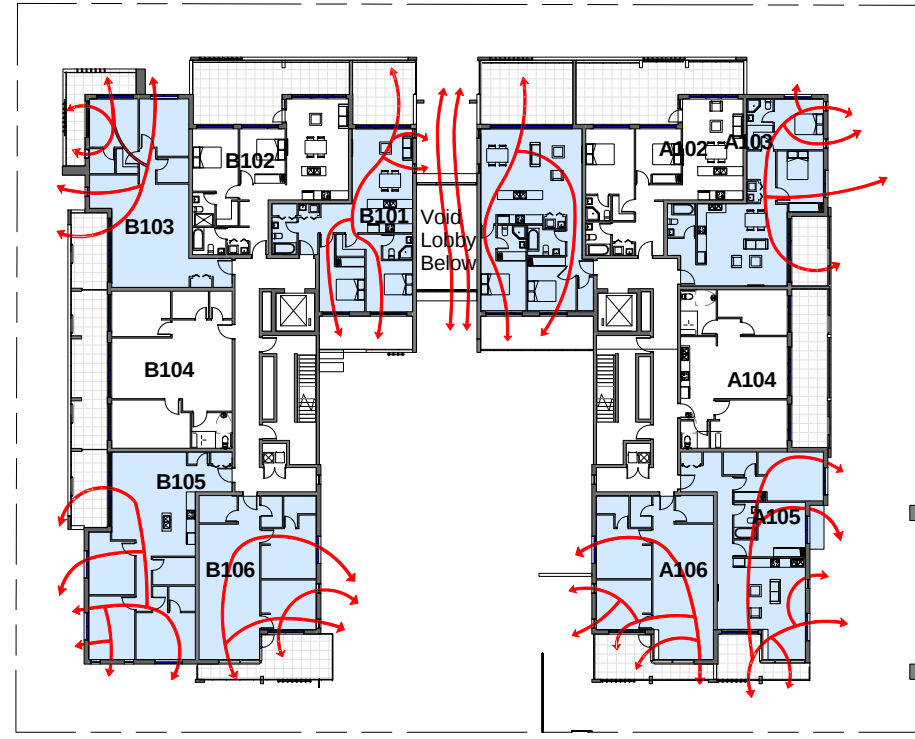
7 Natural Ventilation_Level 1 1 : 500
