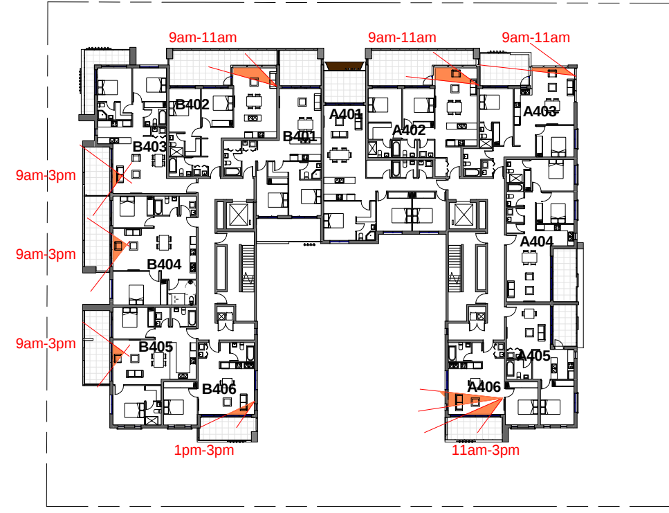
4 Solar Access_Level 4-7 1 : 500
