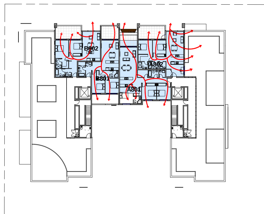
10 Natural Ventilation_Level 8 1 : 500
