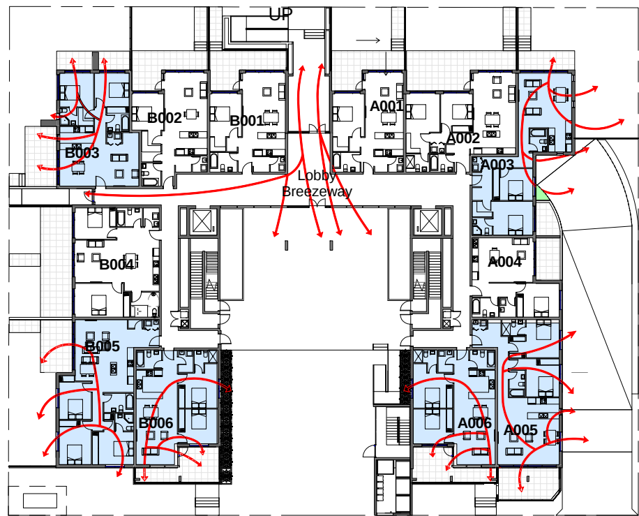
6 Natural Ventilations_Level 0 1 : 500
