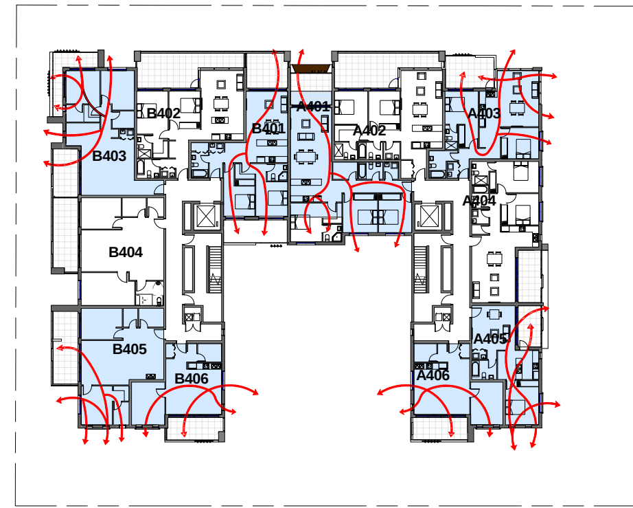
9 Natural Ventilation_Level 4-7 1 : 500
