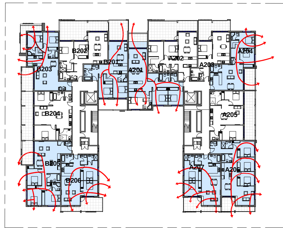
8 Natural Ventilation_Level 2 & 3 1 : 500
